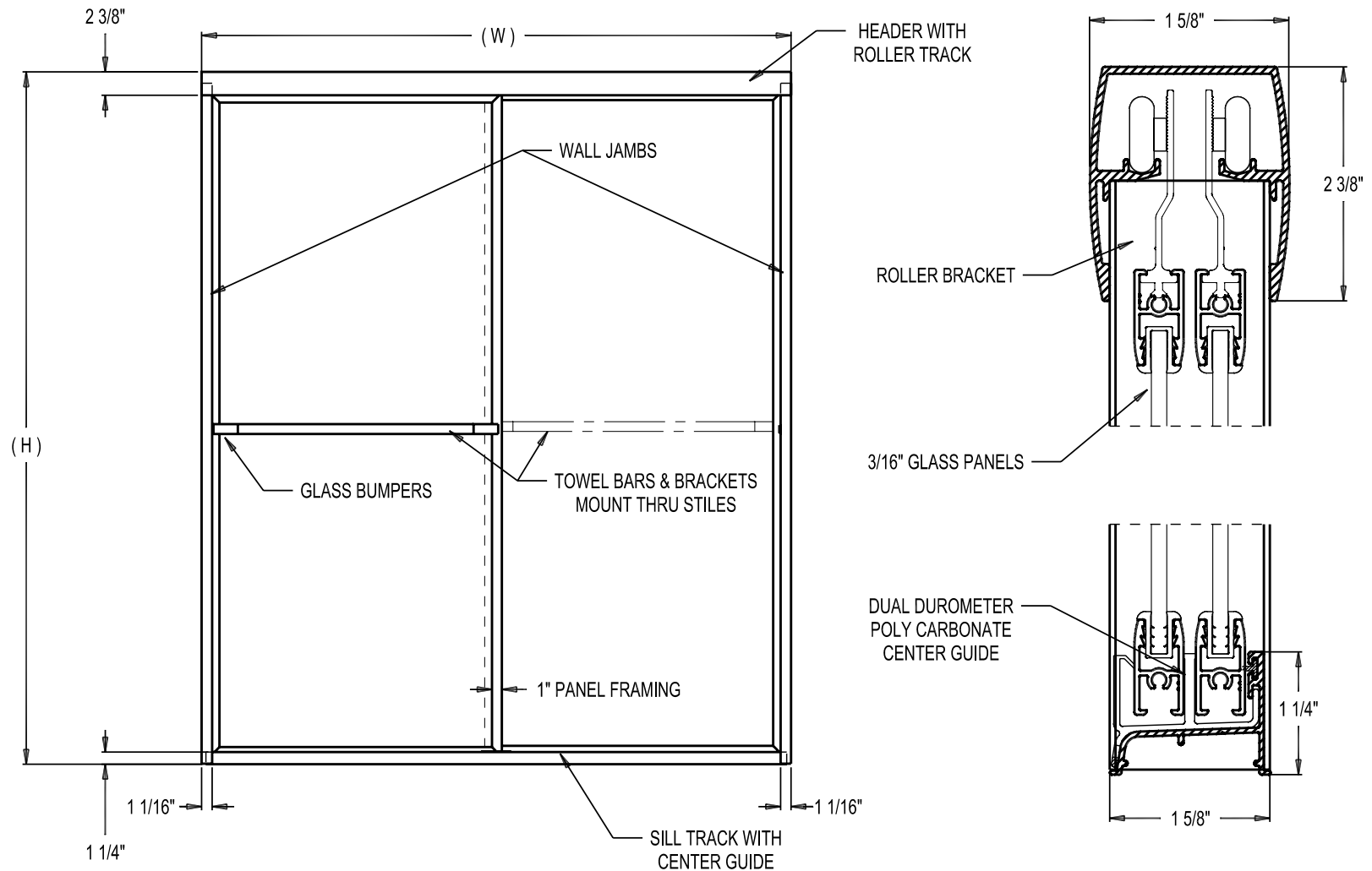
Front Elevation
