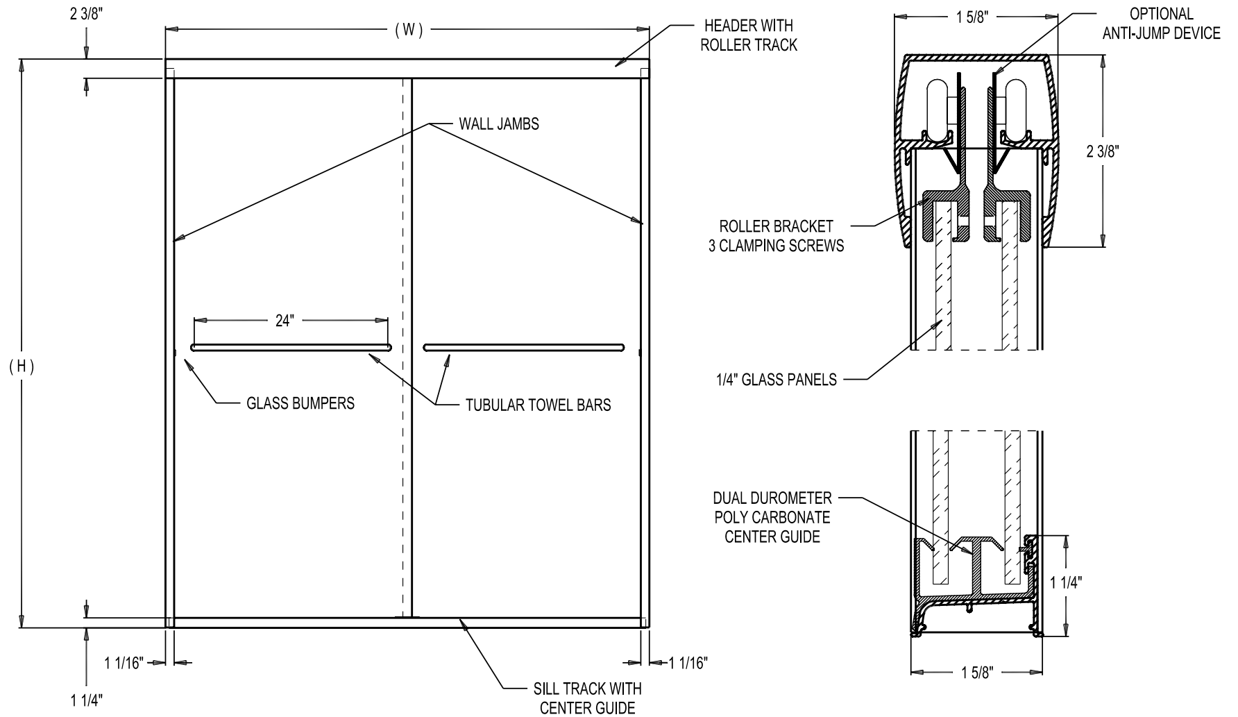
Front Elevation
