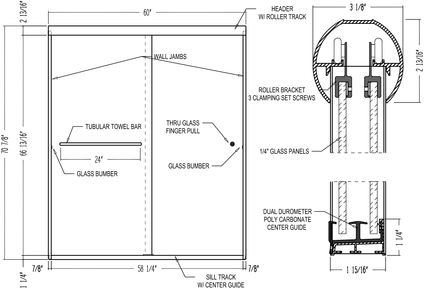
Front Elevation
